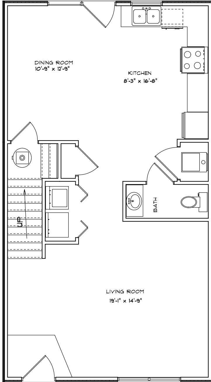
FIRST FLOOR W/SIDING
