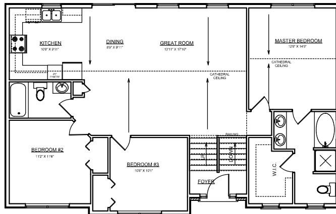
2ND FLOOR LAYOUT
