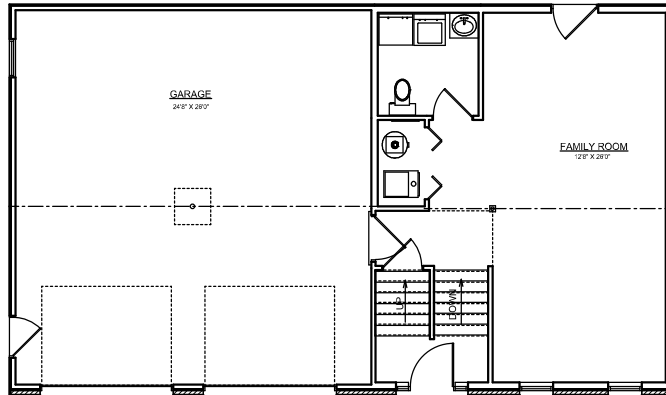
1ST FLOOR LAYOUT
