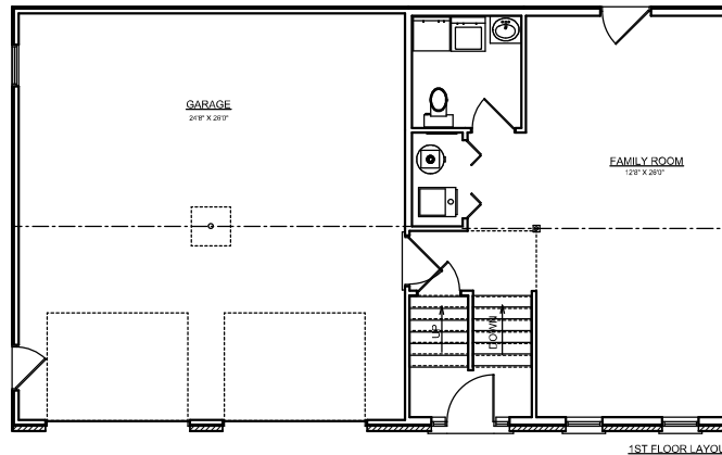
1ST FLOOR LAYOUT
